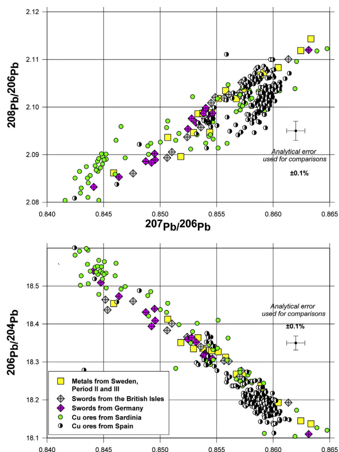
Fig. 16. Lead isotope compositions of Swedish bronze swords from periods II and III and contemporary swords from Germany and the British Isles (Rohl and Needham, 1998) and copper ores from Sardinia and Spain.
