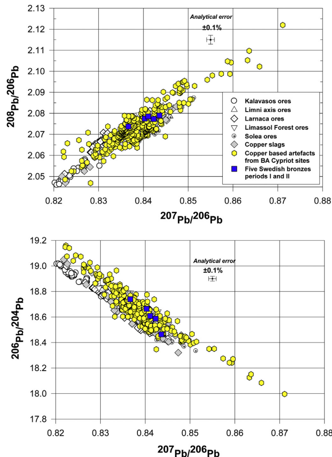
Fig. 13. Lead isotope ratios of five bronzes from Sweden compared with the copper ores from Cyprus and Bronze Age Cypriot copper based artefacts. Not all Bronze Age metals found on Cyprus are made of Cypriot copper: some of them are made of metal from the Taurus Mountains in south Turkey, and some of copper brought from the Western Mediterranean (Stos-Gale and Gale, 2010).
