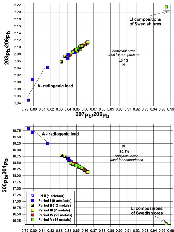
Fig. 9. Mirror image lead isotope plot of all analysed Swedish artefacts. A single data point which plots in the far right corner on both diagrams corresponds to one piece of copper slag from Botkyrka (T1:59; period V). This isotopic signature is consistent with the origin from the Early Proterozoic Bergslagen ores in Sweden (Ling et al., 2013). The data for the three axes dated to Period I in the far left of the plots shows the data for 'radiogenic' lead isotope ratios.
