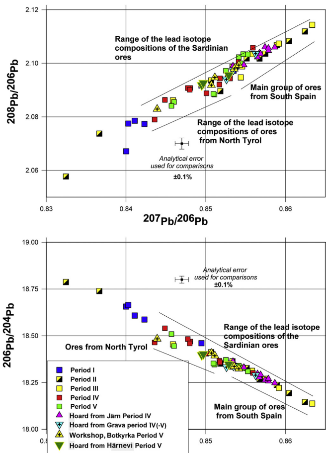
Fig. 15. Lead isotope compositions of artefacts from hoards and a workshop site compared with the other analysed artefacts and approximate range of lead isotope ratios for ore deposits that are consistent with their origin. The lead isotope ratios of the metals from hoards form on the whole compact groups, which might indicate that they are made of recycled, homogenised, metal. However, their lead isotope ratios indicate that in periods IV and V the metal from Spain and Sardinia was predominant.
